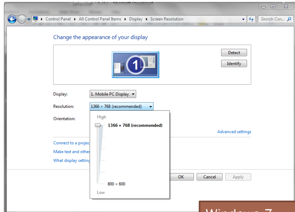
Windows 7
