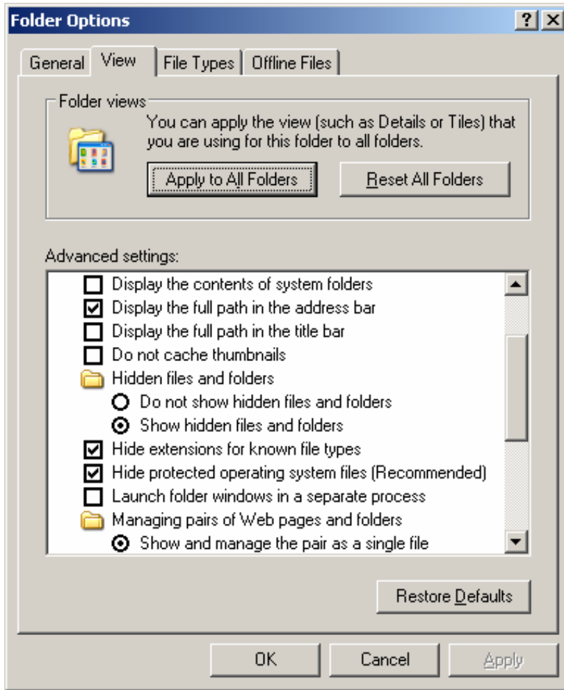
Windows 98
